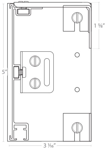
URBAN 5 RETURN 3 Showing all hardware
