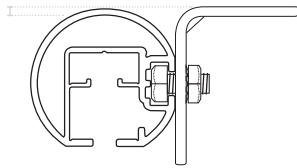
CEILING SUPPORT
