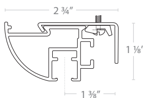
INVISIBLE SHORT PROJECTION SUPPORT
