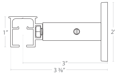
WALL SUPPORT
