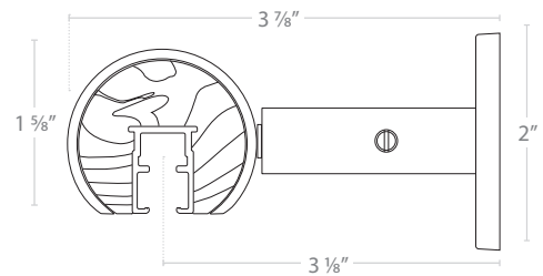
WALL SUPPORT
