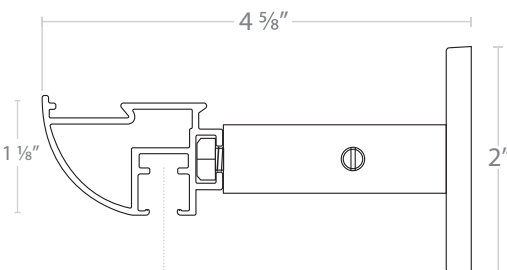
INVISIBLE TEKNO 2" PROJECTION for Tekno 4" - add 2" for measurements from wall
