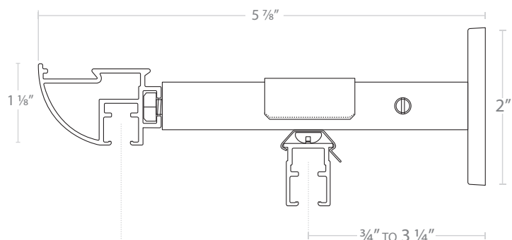
INVISIBLE TEKNO 4" PROJECTION WITH EURO SCOPE UPGRADE for Tekno 6" projection - add 2" for measurements from wall
