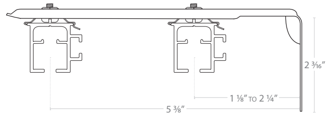
DOUBLE SUPPORT
