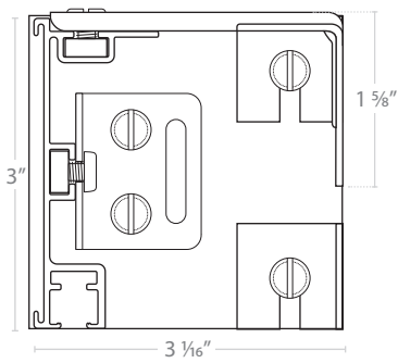
URBAN 3 RETURN 3 Showing all hardware
