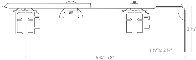
ADJUSTABLE DOUBLE SUPPORT
