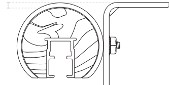
CEILING SUPPORT
