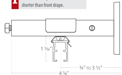
EURO-SCOPE INSTALLATION 4" Support shown
