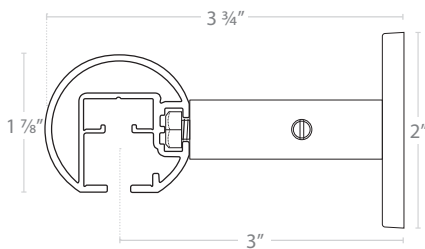
WALL SUPPORT
